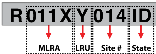
Figure A5.2. Components of an ecological site description code. "R" at the beginning of the code denotes a rangeland ecological site.
