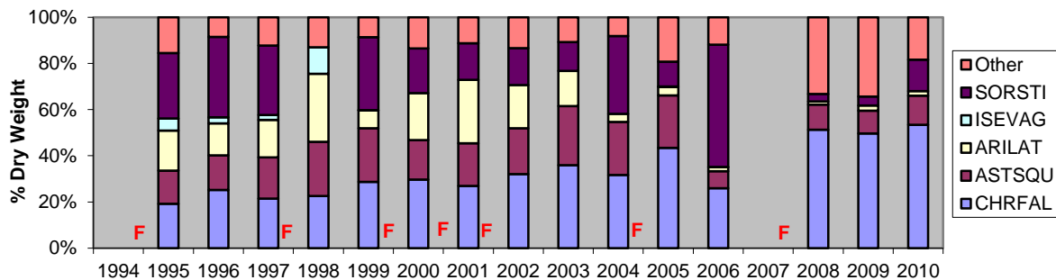
Fig. 4. Pasture composition at site F8, showing fires (F). Species are: Sorghum stipoides , Iseilema vaginiflorum , Aristida latifolia , Astrelba squarrosa and Chrysopogon fallax .
