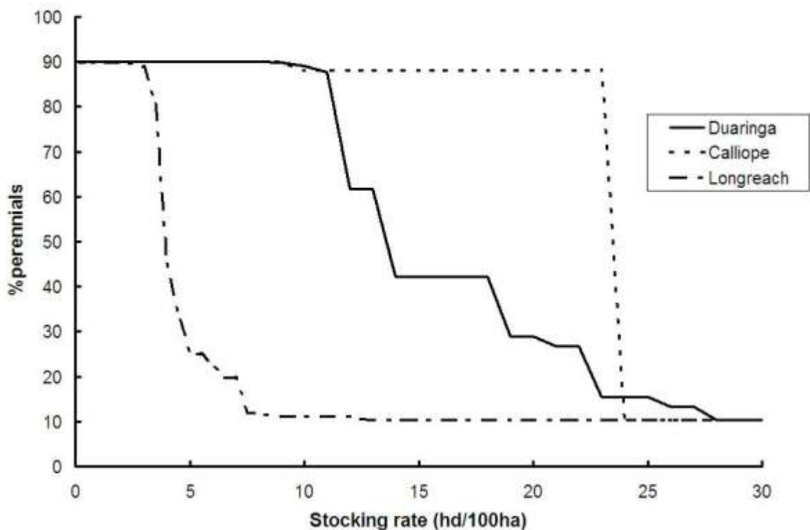
Fig. 2. Simulated percent perennials in pasture for an infertile land type at a range of stocking rates for three different climate locations. Note: same parameter set used for all simulations, with only the climate station changing.
