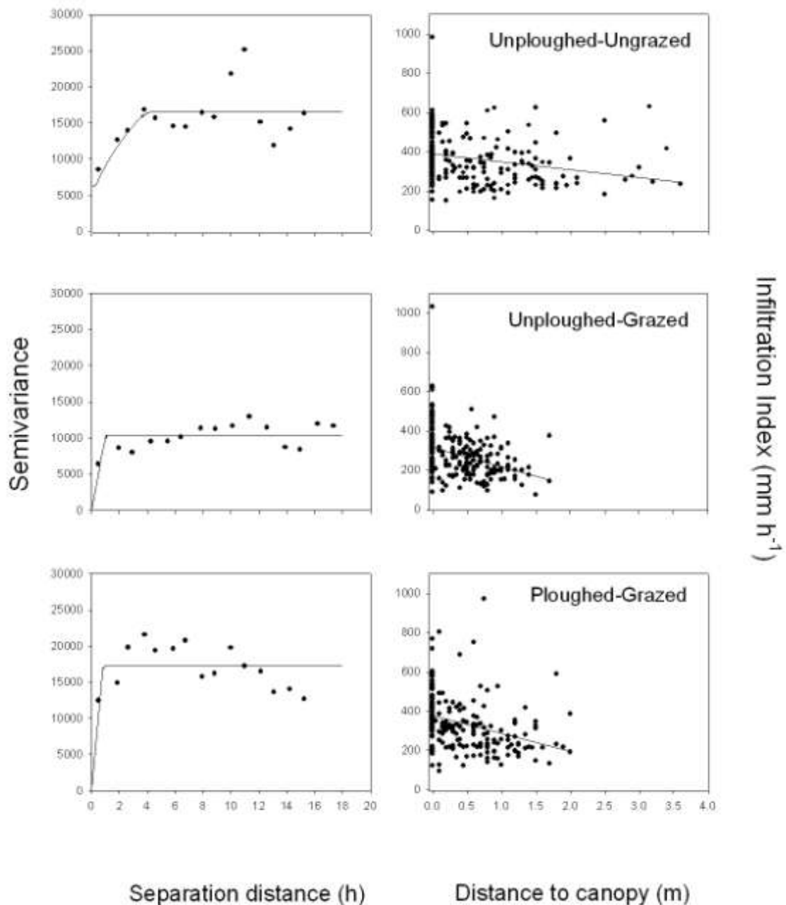
Fig. 1. Semi-variogram of infiltrability as well as relationship between distance to canopy and infiltration at three different sites
