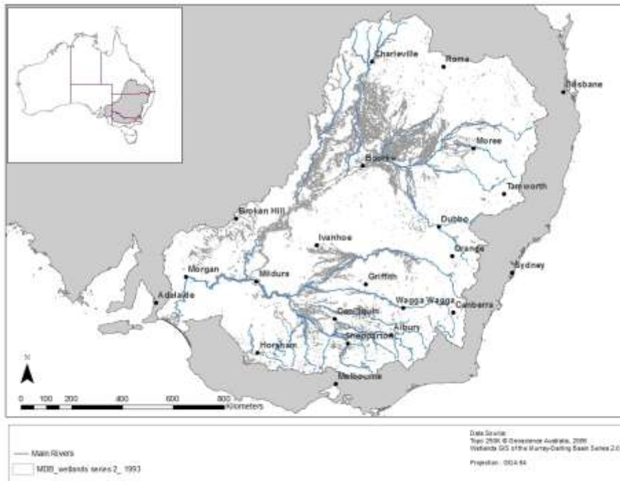
Figure 1. Extent of floodplain wetlands in the MDB.
