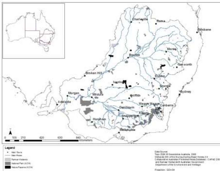
Figure 2. RAMSAR Wetlands and Nature Resources in the MDB.
